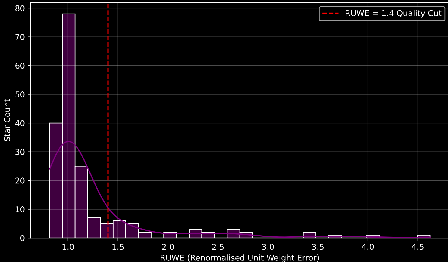
GAPOGEE DR17 Field [201+29] RUWE Distribution (n= 185)
